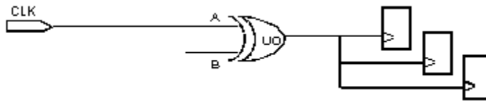
Figure 36 Non-Unate Gated Clock
