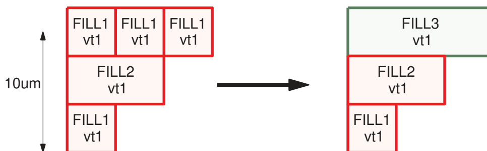
Figure 95 Fixing Maximum Stacking Violation by Replacement
