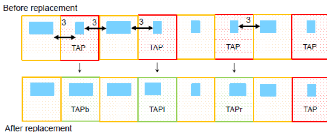
Figure 98 Fixing a Tap Cell Spacing Violation
