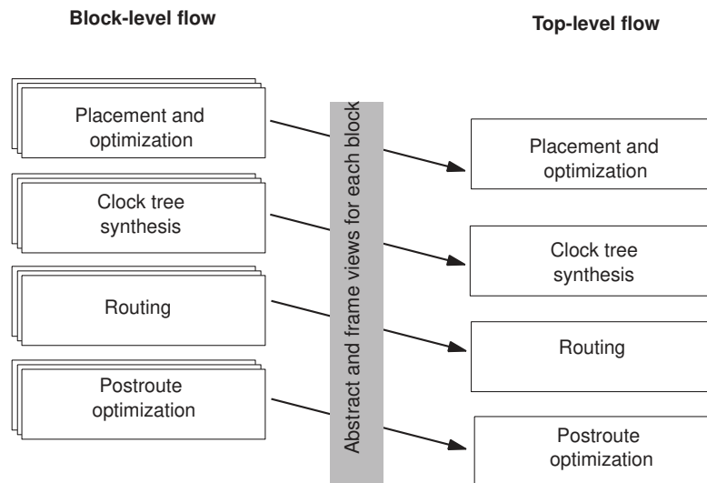
Figure 156 Top and Block Levels Implemented in Parallel
