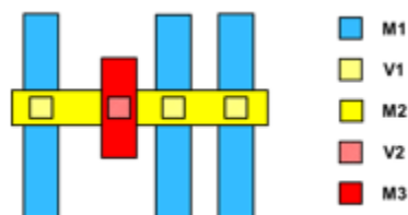
Figure 75 Multi-Level Pattern-Based Must-Join Pin Connection
