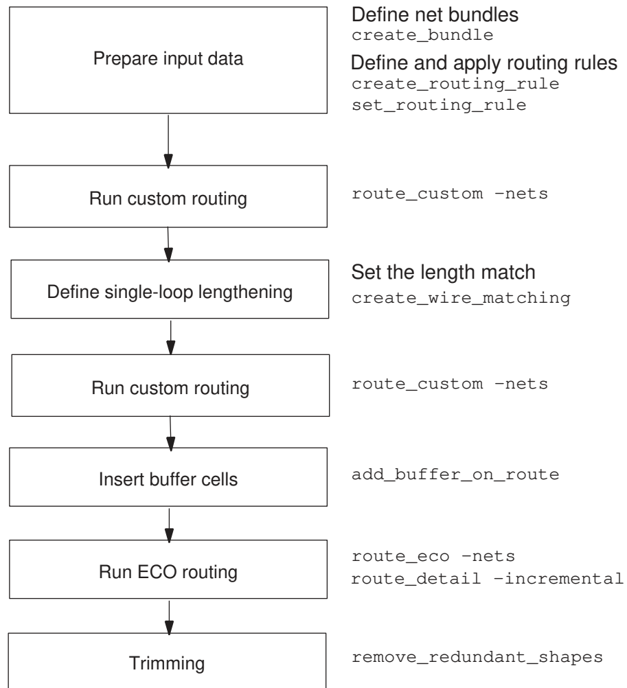
Figure 129 A Basic DDR Flow
