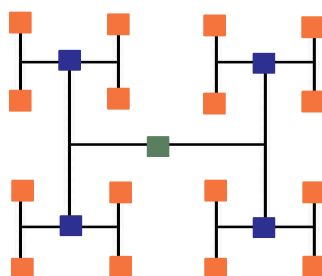
Figure 52 Clock Drivers Placed in an H-Tree Structure
