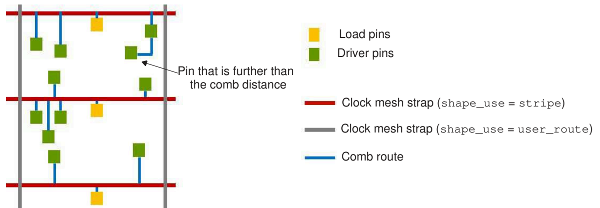
Figure 58 Comb Topology
