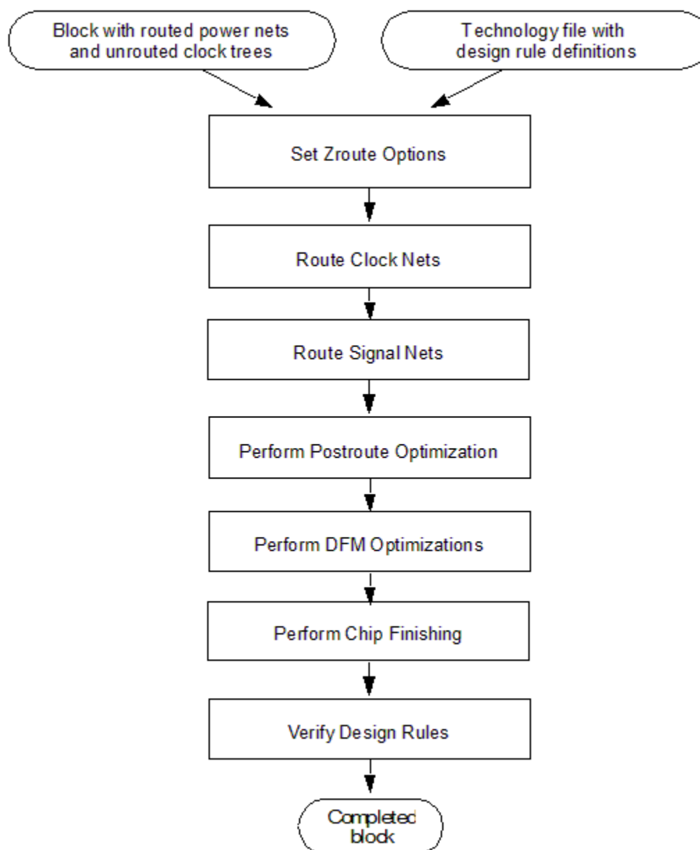
Figure 63 Basic Zroute Flow
