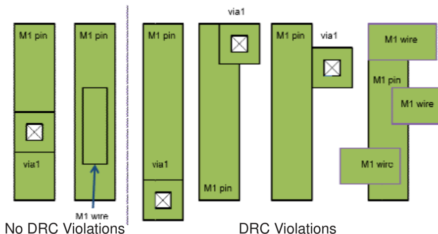
Figure 79 Restricted Via-to-Pin and Wire-to-Pin Connections
