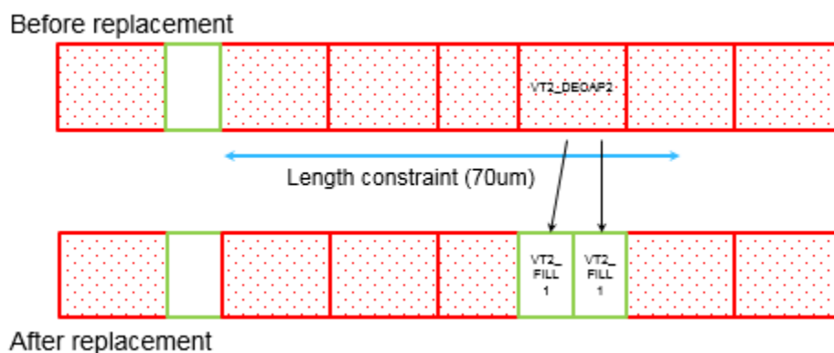
Figure 94 Fixing a Maximum Vertical Edge Length Violation
