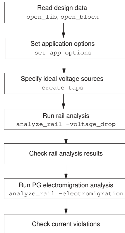
Figure 160 Required Steps for a Basic Rail Analysis Using RedHawk and RedHawk-SC Fusion
