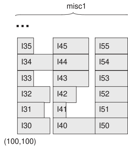
Figure 137 Anchored Relative Placement Group
