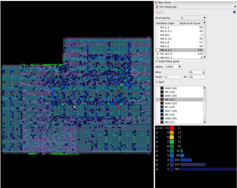
Figure 107 Selecting Layers in the ICV Heatmap
