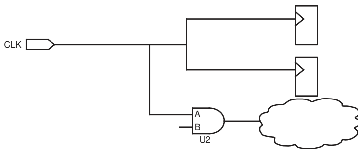
Figure 39 User-Defined Ignore Pin
