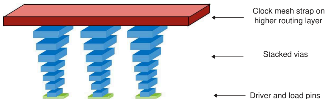
Figure 59 Vias in the Comb Topology
