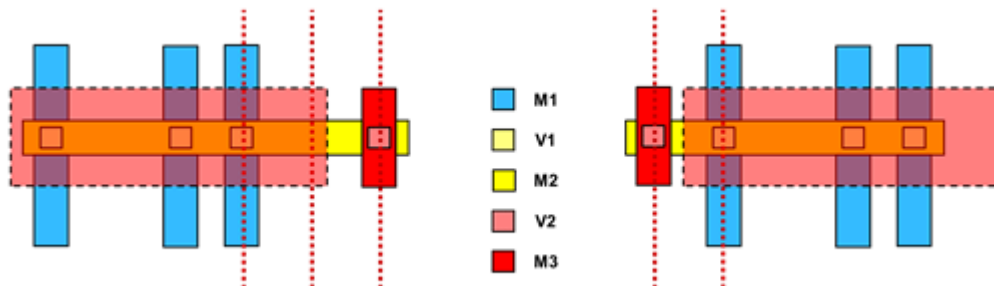
Figure 76 Pattern-Based Must-Join Pin Connection With Staggering
