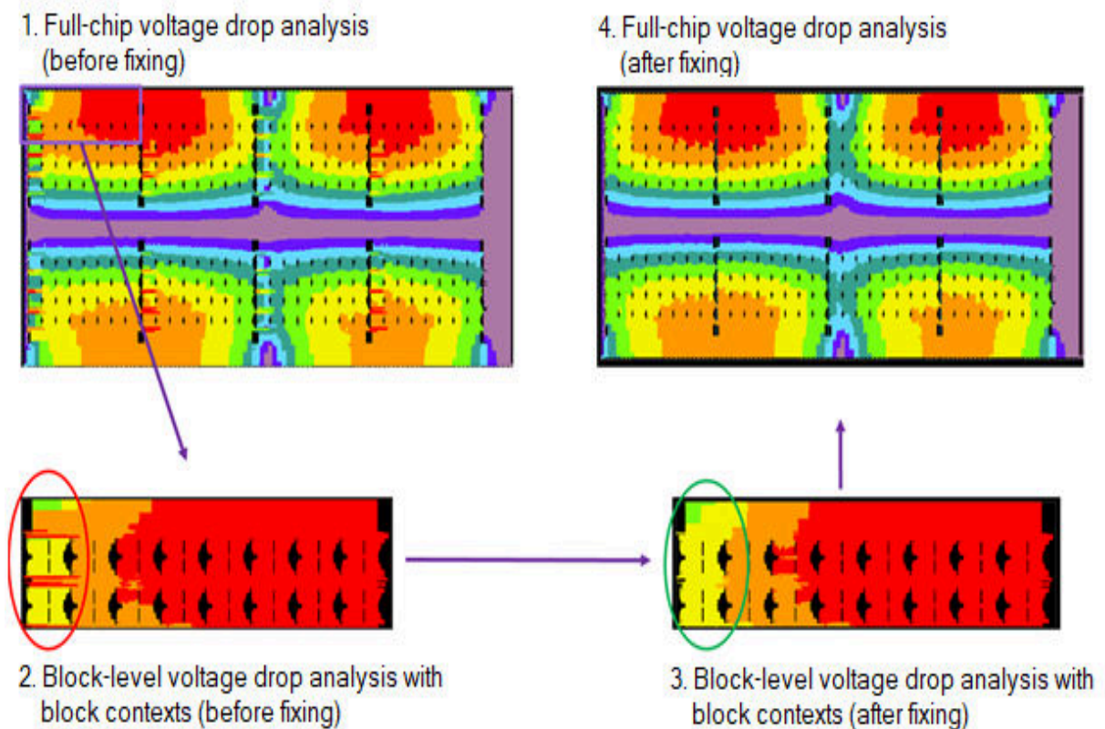
Figure 171 Fixing Violations in Block Contexts
