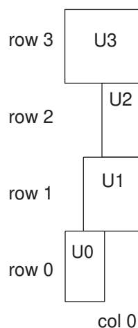
Figure 143 Right-Aligned Relative Placement Group With One Cell That is Left Aligned
