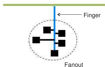
Figure 56 Fanout of a Finger of the Fishbone Topology
