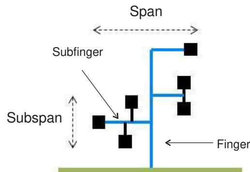
Figure 57 Span and Subspan of the Fishbone Topology
