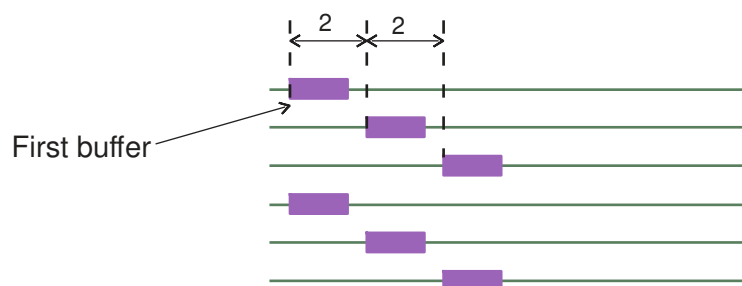
Figure 179 Buffer Patterns for a Horizontal Bus
