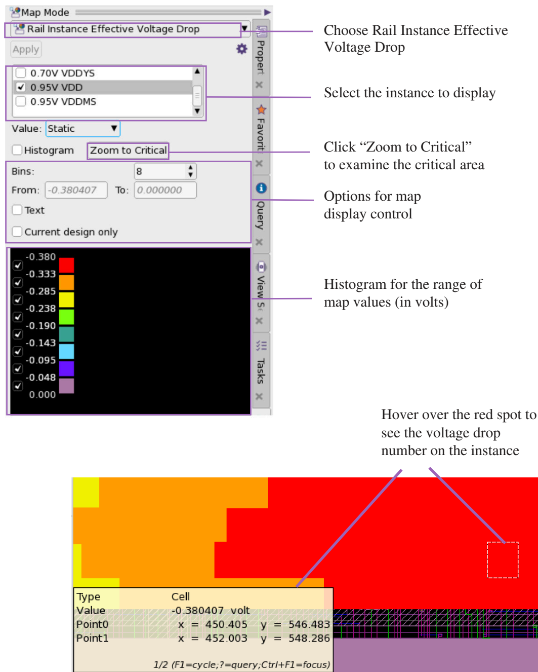
Figure 172 Displaying a Rail Instance Effective Voltage Drop Map
