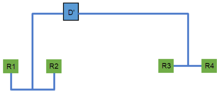
Figure 122 Receivers With Matched Wire Length From Driver D'
