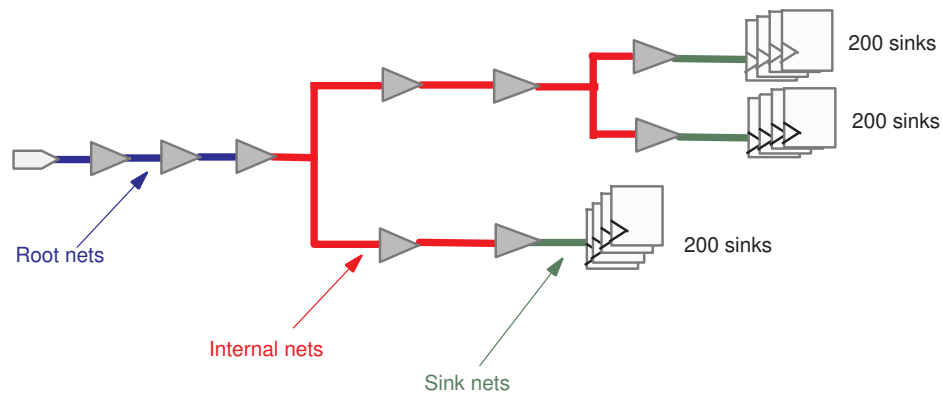
Figure 71 Root, Internal, and Sink Clock Net Types
