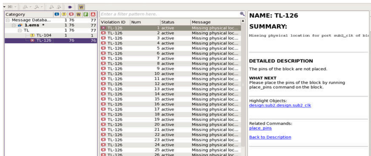
Figure 154 Viewing the EMS Database in the Message Browser
