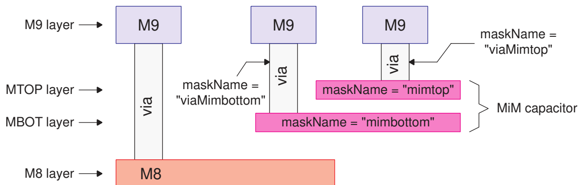
Figure 91 Cross-Section View of MiM Capacitor Layers
