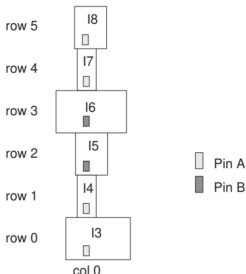
Figure 142 Relative Placement Group Aligned by Different Pins
