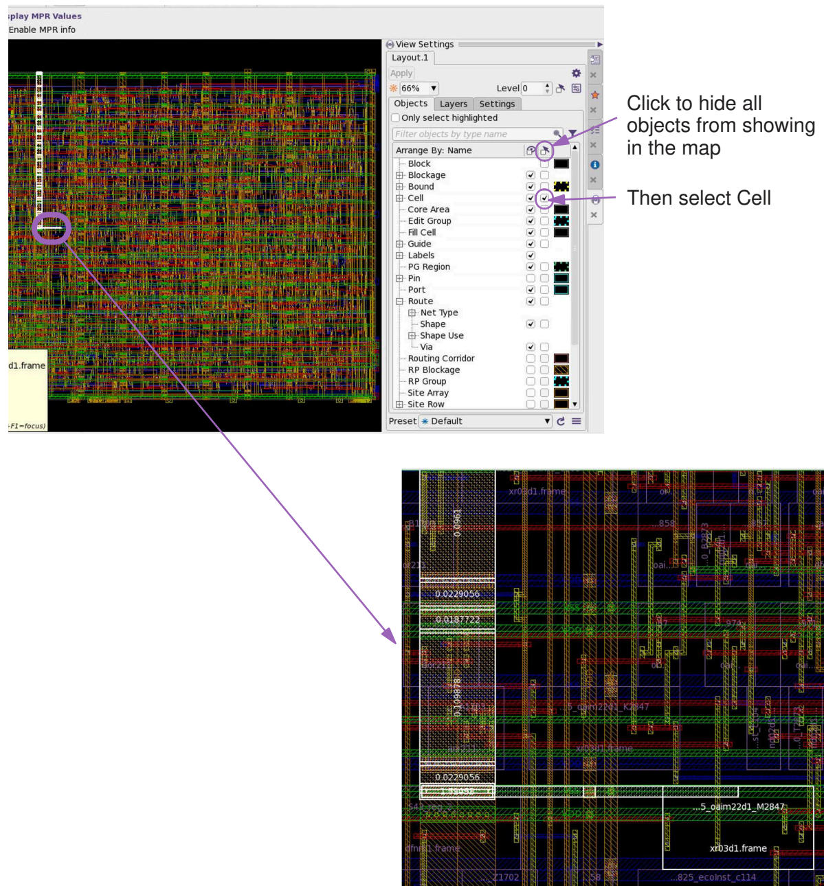
Figure 169 Tracing the Path With the Least Resistance
