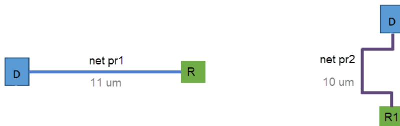
Figure 119 Minimum Wire Length Constraint for pr* Nets
