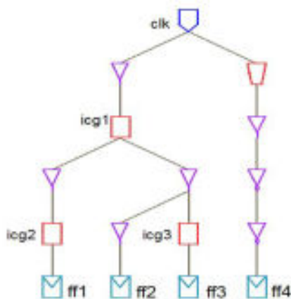
Figure 62 Segments and Subtrees of a Clock Tree
