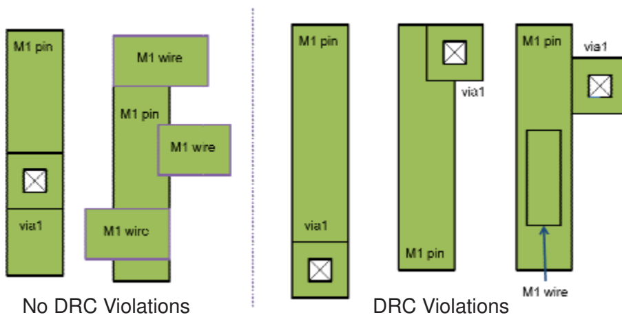
Figure 78 Restricted Via-to-Pin Connections
