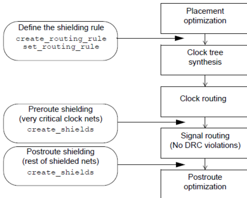
Figure 81 Zroute Shielding Flow
