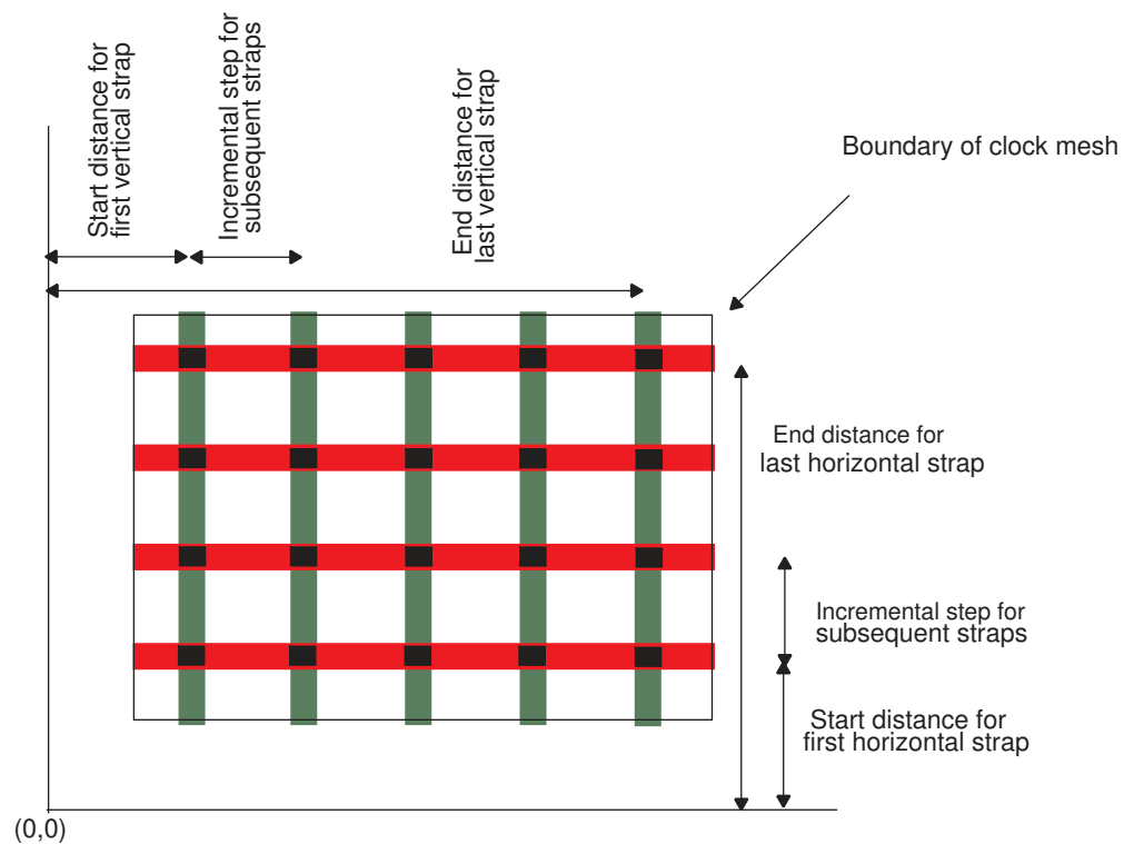
Figure 53 Clock Mesh Structure
