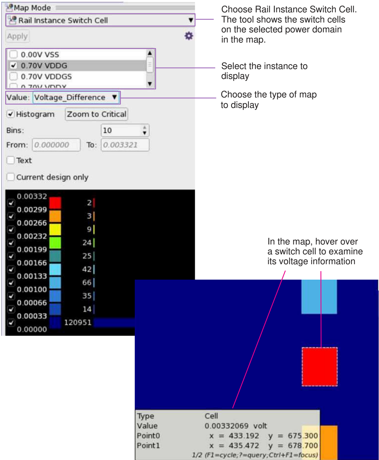
Figure 173 Displaying Maps for Switch Cells
