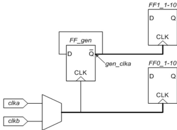
Figure 42 Clock Pins That Cannot Be Balanced Simultaneously
