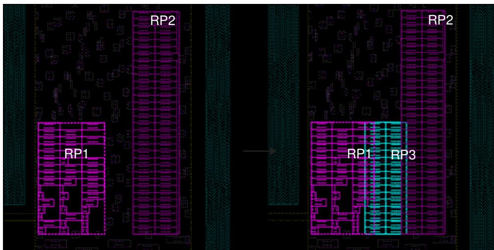
Figure 150 Legalizing the RP3 Relative Placement Group Over Other Groups
