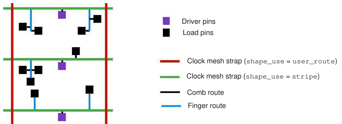
Figure 55 Fishbone Topology
