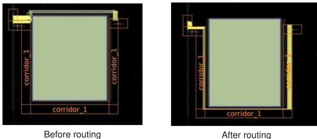
Figure 69 Using a Routing Corridor
