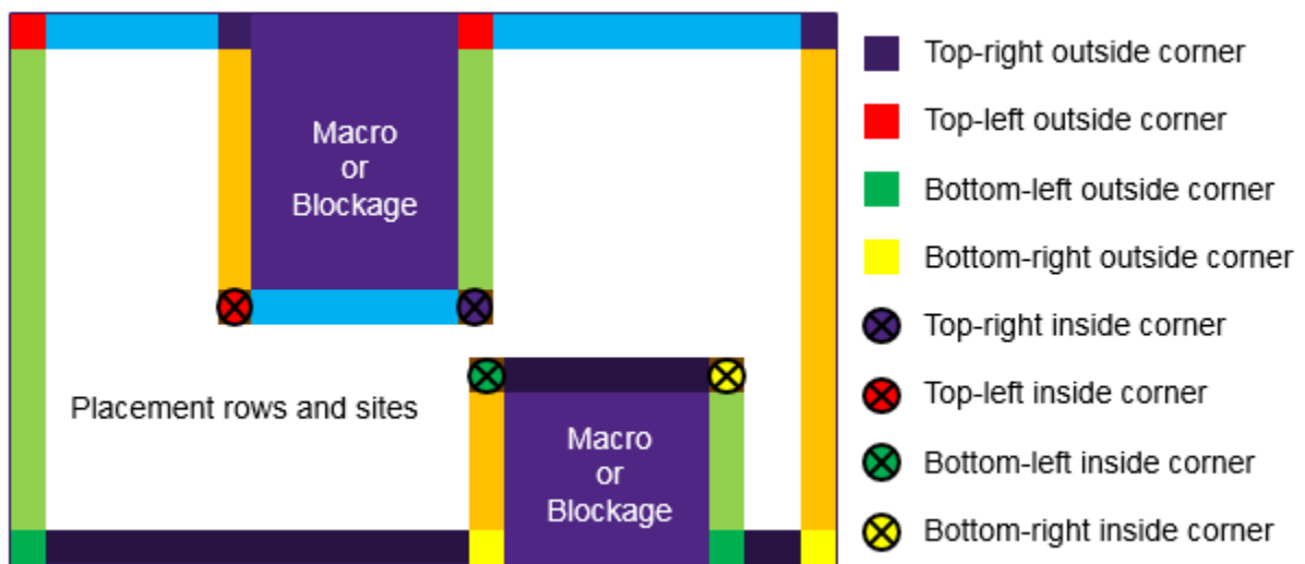
Figure 87 Boundary Cell Locations
