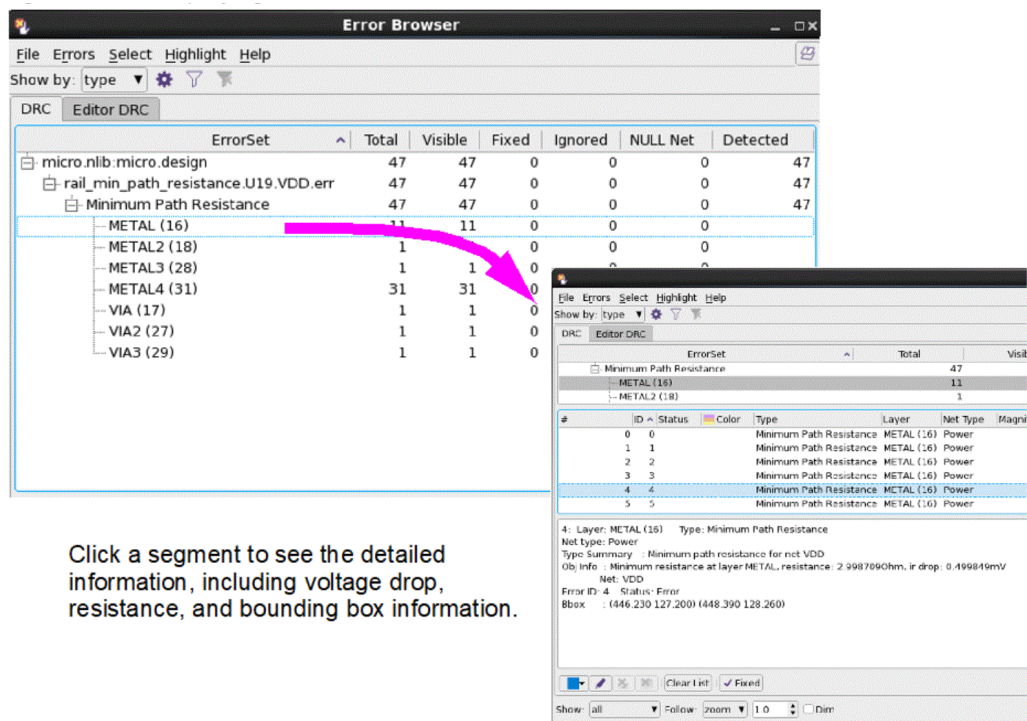
Figure 166 Displaying Error Cells in the Error Browser
