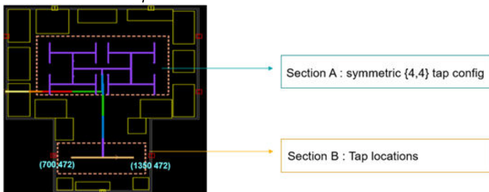
Figure 51 MSCTS Multiple H-Tree
