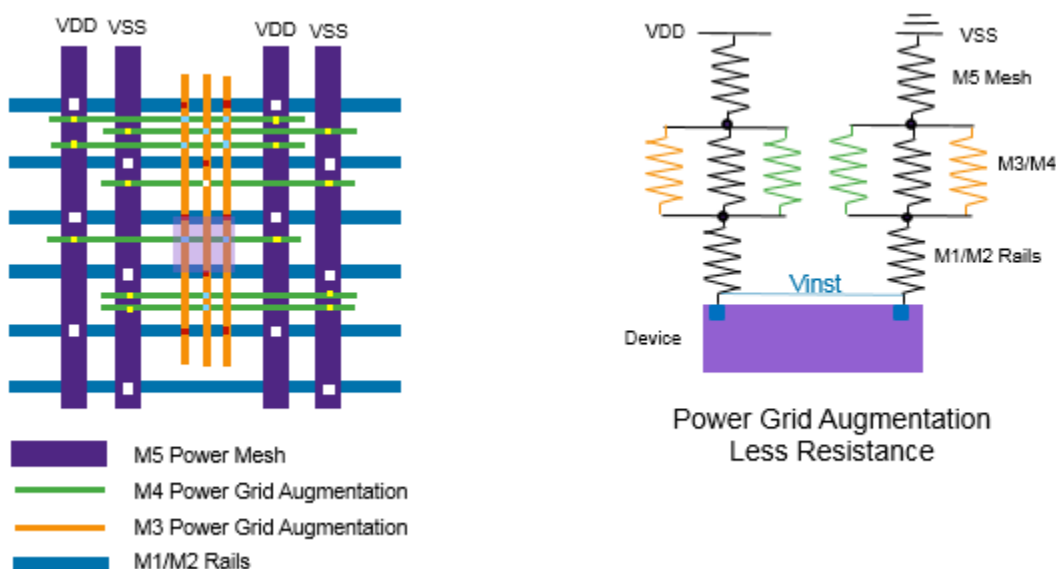
Figure 112 Power Grid Augmentation
