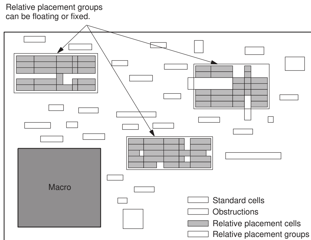
Figure 130 Relative Placement in a Floorplan
