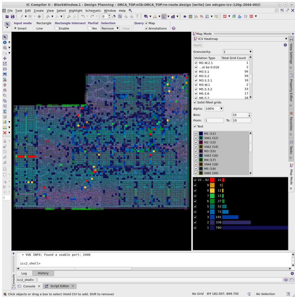
Figure 99 ICV Heat Map
