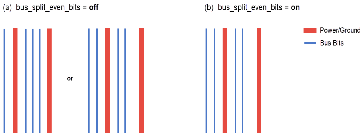
Figure 127 Splitting Bus Trunk to Route Through Power and Ground Rails
