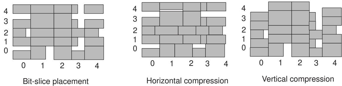
Figure 144 Bit-Slice Placement Versus Horizontal or Vertical Compression
