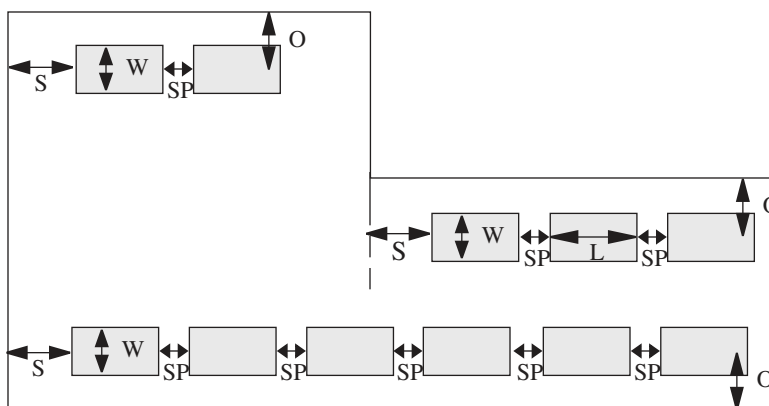
Figure 66 Metal Stub Perimeter Constraint Objects
