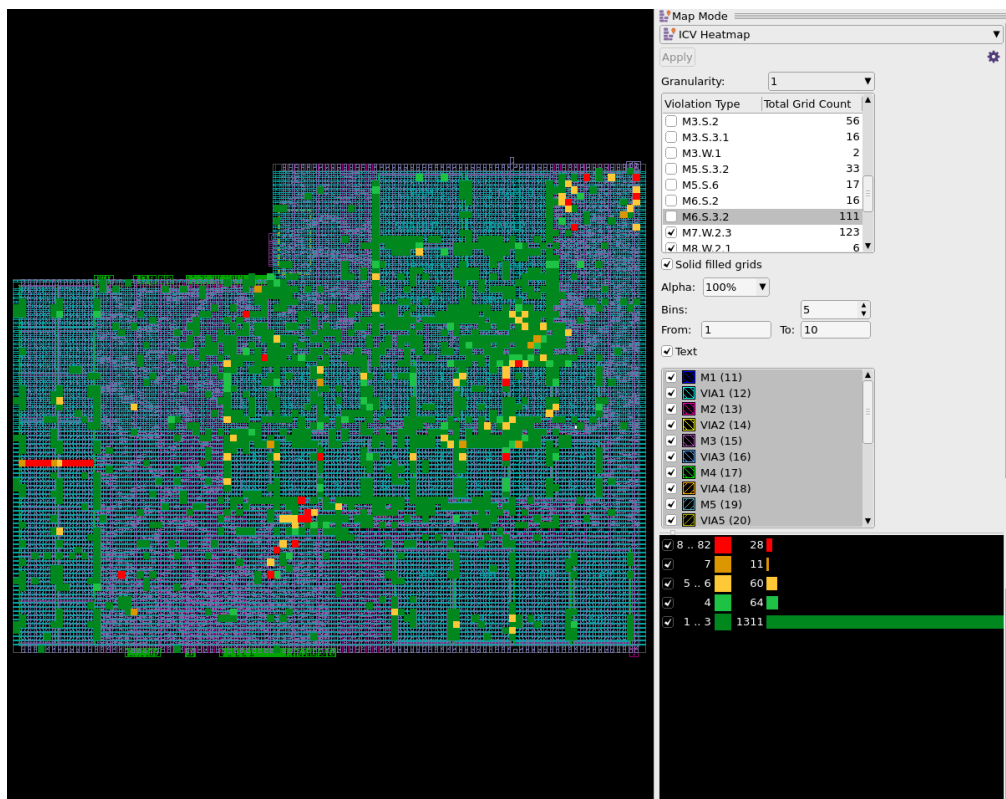
Figure 104 Bins Value Set to 5
