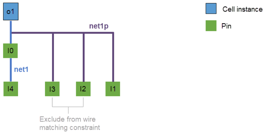
Figure 126 Net-Based Wire Matching Constraints With Pin Exclusions
