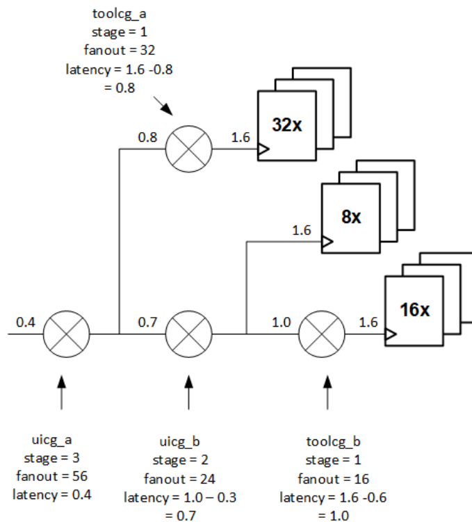
Figure 16 Latency Calculations With Varying Fanout
