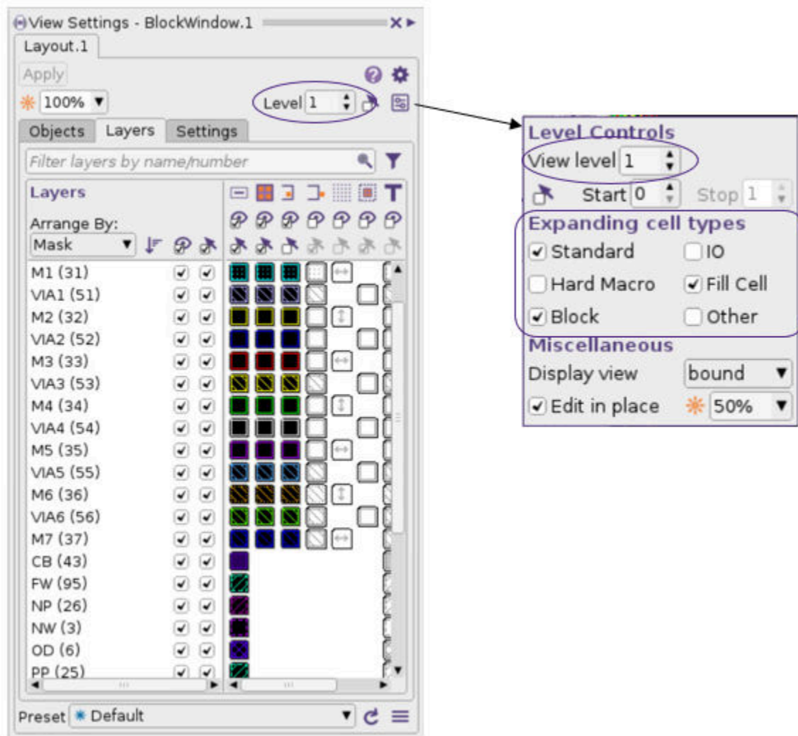
Figure 110 Settings Used to Display Objects for Design Rule Checking
