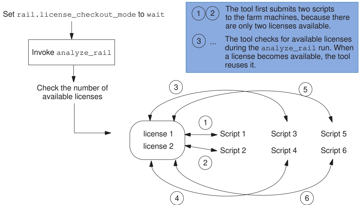
Figure 170 Waiting for Available Licenses During Distributed RedHawk Fusion Run
