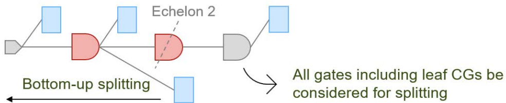
Figure 45 Latency Driven Clock-Gate Splitting
