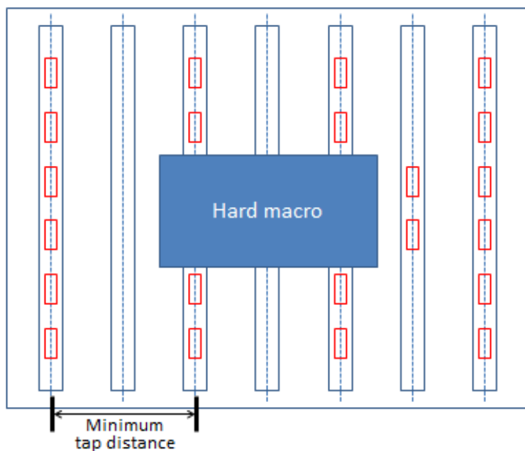
Figure 85 Default Tap Cell Placement
