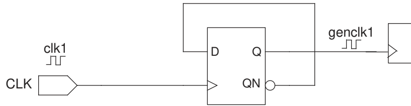
Figure 37 Nested Clock Tree With a Generated Clock
