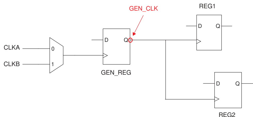
Figure 43 Generated Clock With Invalid Master Clock Source
