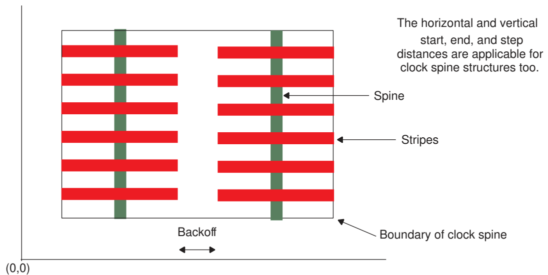
Figure 54 Clock Spine Structure
