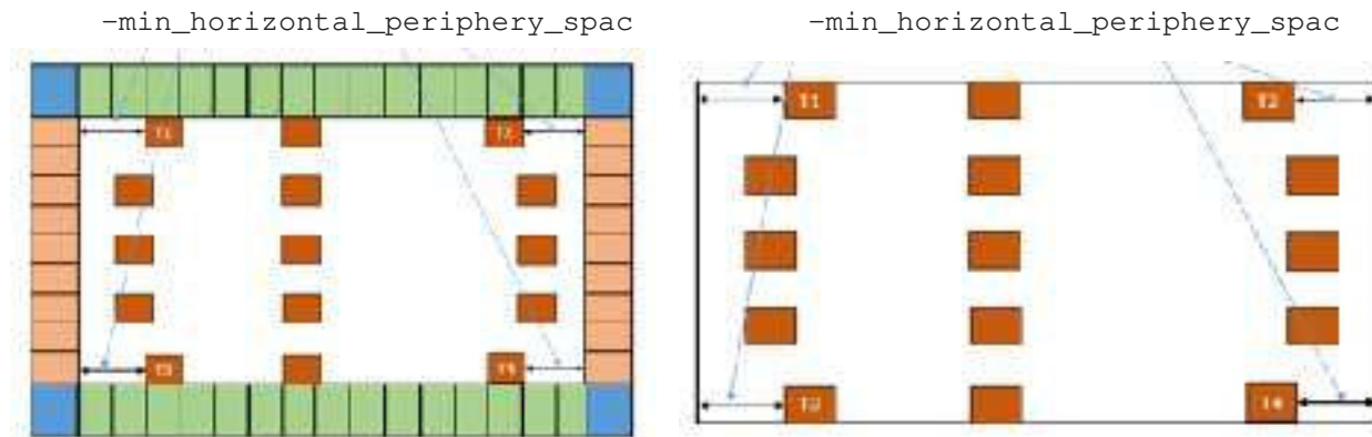
Figure 86 Tap Cell Boundary Row Spacing
