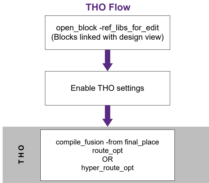
Figure 157 Transparent Hierarchy Optimization Flow
