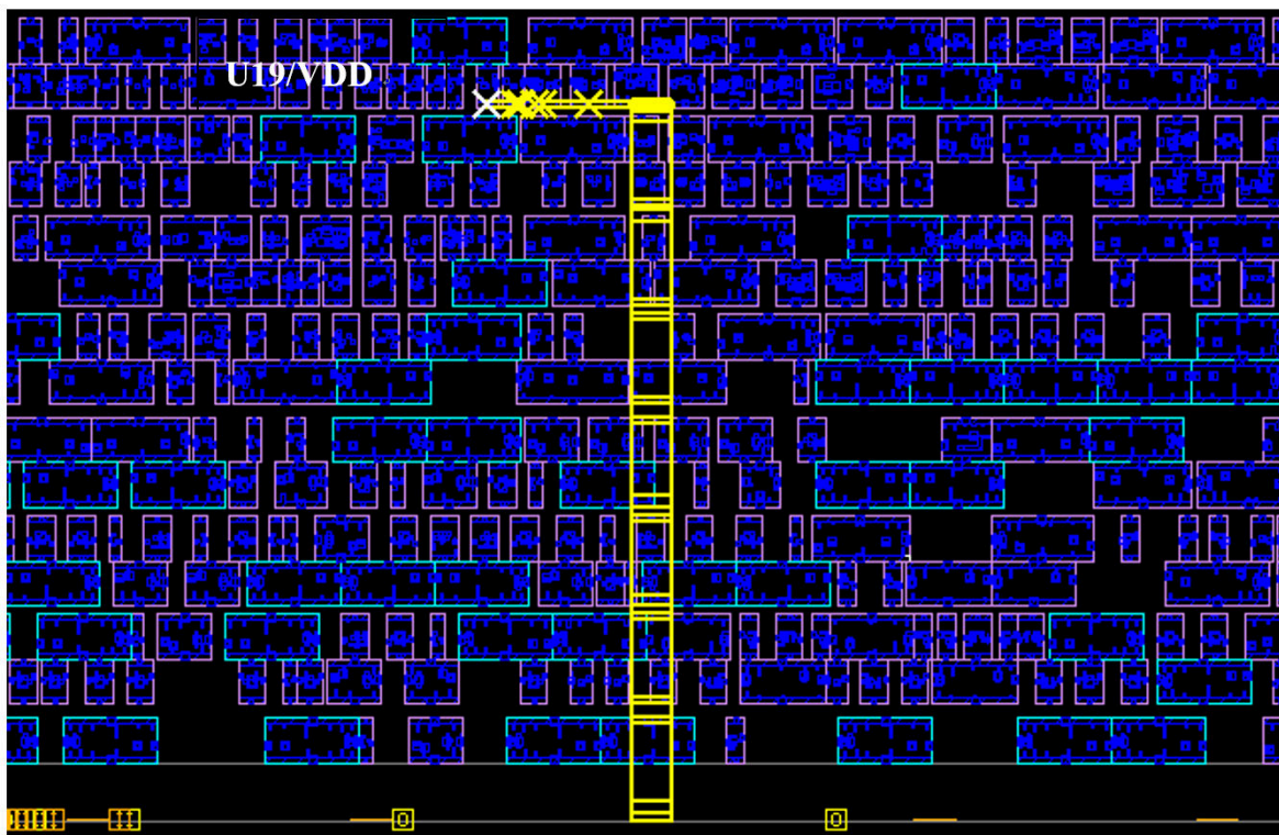
Figure 167 Traced Segment is Highlighted in the Design Layout
