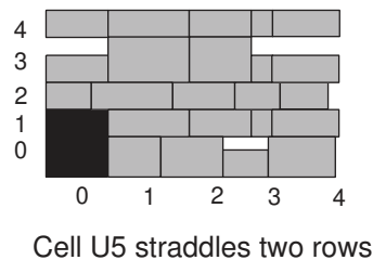
Figure 145 Compression of a Relative Placement Group With a Cell That Straddles Multiple Rows
