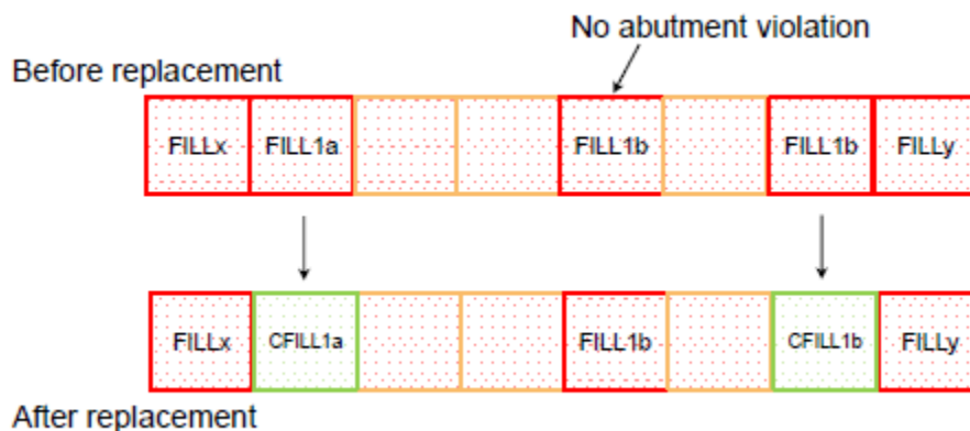
Figure 93 Fixing an Illegal Abutment Violation
