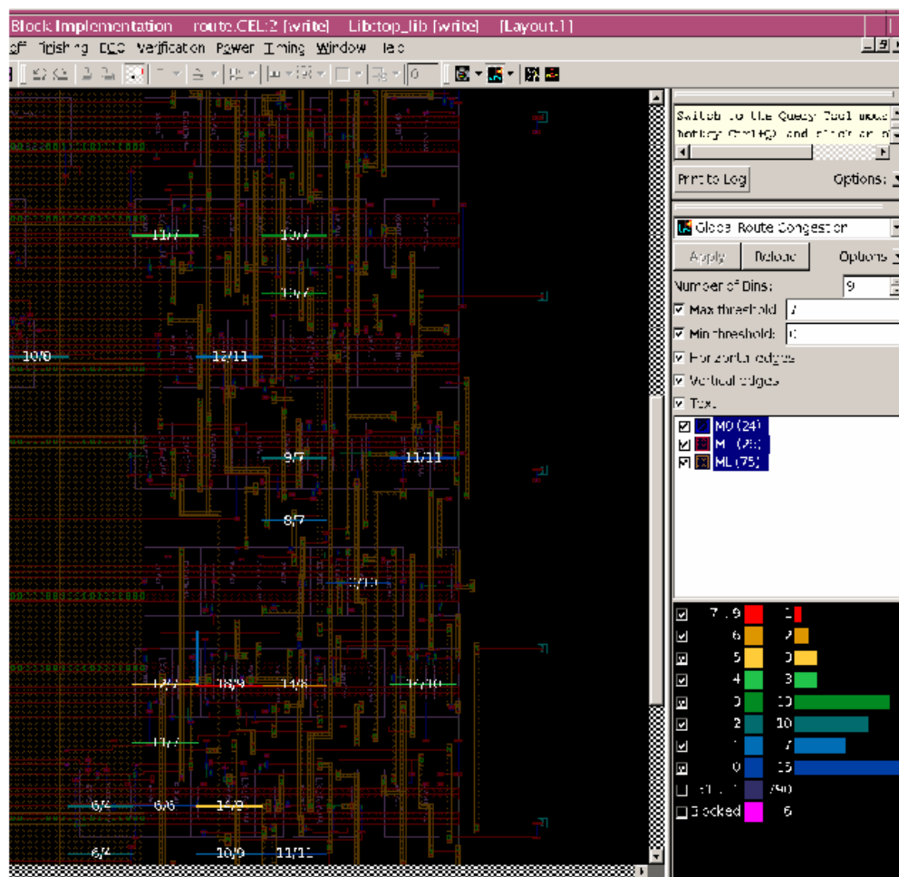
Figure 83 Global Route Overflow on Global Routing Cell
