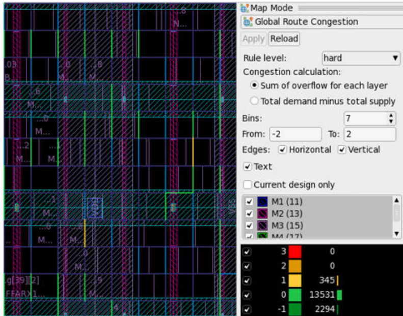
Figure 82 Global Route Congestion Map
