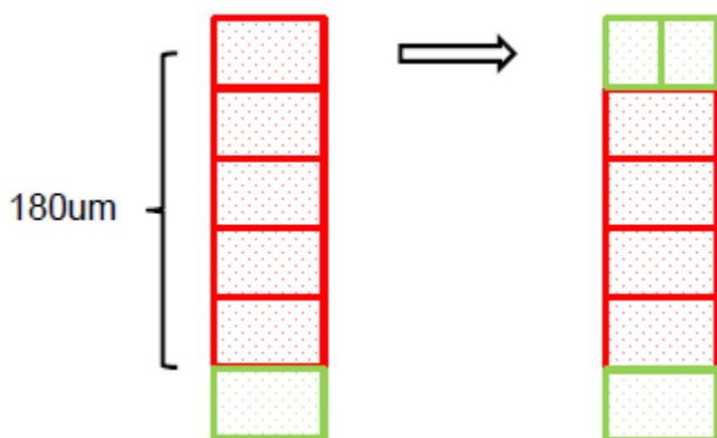
Figure 97 Fixing a Maximum Vertical Edge Length Violation
